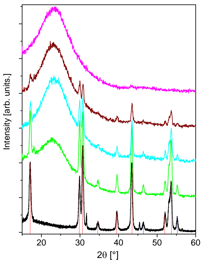
Figure S5: XRD-spectra of oleate-coated UNCP cores ( 24 \pm 2 nm diameter, sample C1, black line) where red bars indicate reference values of the hexagonal phase (JCPDS No.00-028-1192) and blue bars indicate reference values of the cubic phase (JCPDS No. 01-077-2042), and XRD spectra of the same cores after the second silica coating (C1_2S, shell thickness: 18 \pm 2 nm, green line), third silica coating (C1_3S, shell thickness 35 \pm 2 nm, cyan line), fourth shell silica coating (C1_4S, shell thickness: 44 \pm 2 nm, brown line), and fifth silica coating (C1_5S, shell thickness: 149 \pm 8 nm, pink line).
