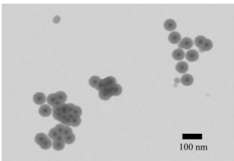
Figure S3: STEM image of UCNP (sample C1, 24 \pm 2 nm diameter) which were coated in a four-step silica shell process in a reverse microemulsion process with an R-value or 1:2.2, which leads to the formation of core-free silica particles due to a too high ammonia water concentration, which accelerates the hydrolysis rate of TEOS. The size of the silica-coated UCNPs was 107 \pm 6 nm, and the core-free particles had an average diameter of 60 \pm 15 nm.
