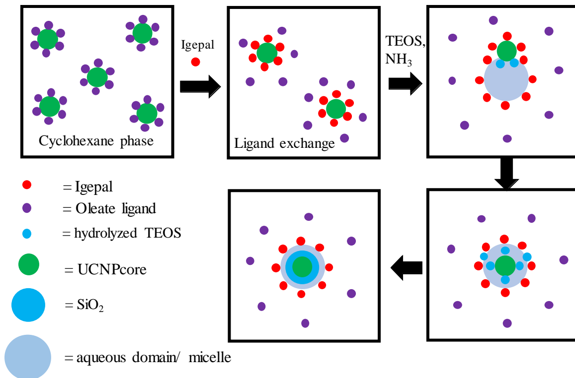
Figure S1: Scheme of microemulsion synthesis for coating oleate-functionalized UCNPs with a first thin silica shell. Upon addition of surfactant in the UCNPs dispersion, a ligand exchange between oleate ligands and the surfactant occurs. Upon addition of TEOS and NH 3 , aqueous micelles are formed, and TEOS is hydrolyzed at the interface between the oil (cyclohexane) and the water phase. A second ligand exchange occurs between hydrolyzed TEOS (silica monomers) and Igepal, which transfers the UCNPs into the micelles where the condensation reaction of the silica monomers takes place, leading to the formation of the final silica shell.
